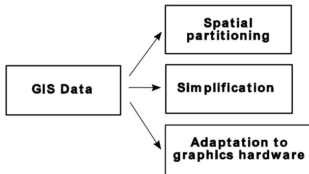
Figure 6: Real-time adapter
