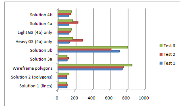
Figure 12: Rendering times (ms) of the proposed solutions for the three test data sets (percentage relative to the best case).
